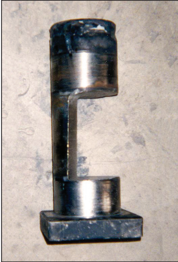
High-Manganese steel pin after 7 days of service. Original pin diameter was 5".
